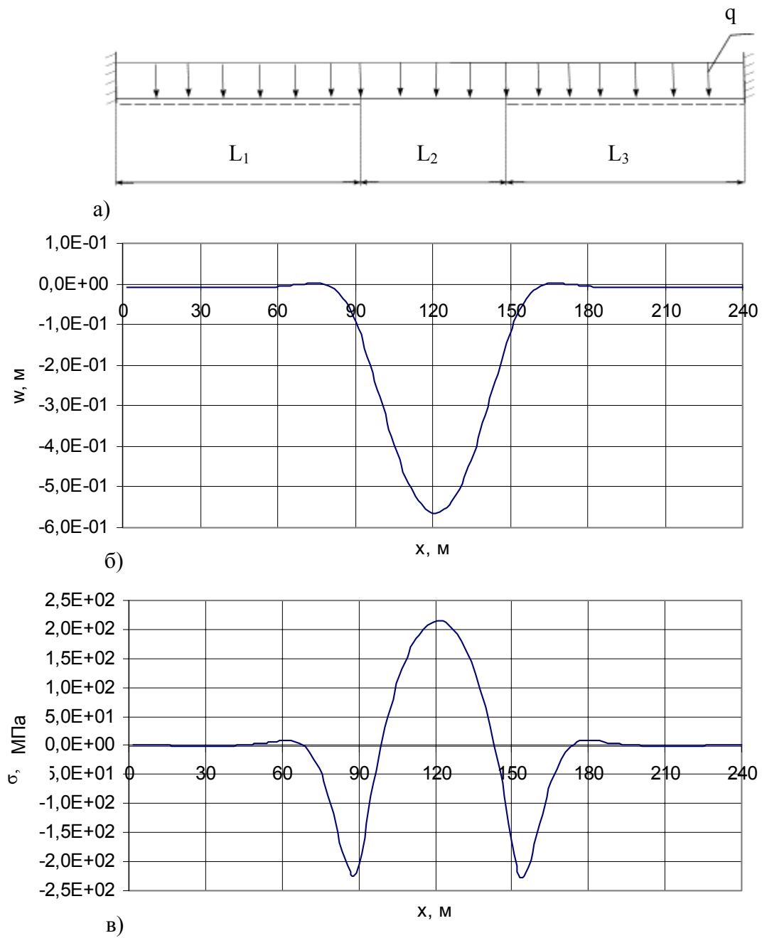
Fig.1 The calculation of main parameters of SDC of the submerged pipeline in the carst zone: a) a designed pipeline diagram ( L_1=L_3=90 m, L_2=60 m; p_0=7,5 Mpa; \Delta t=20 deg.C); b) diagram of saggings; c) bending stresses
