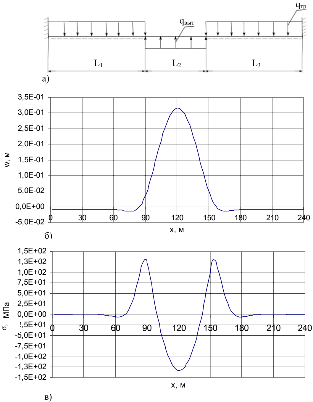
Fig.4 The calculation of main parameters of SDC of the submerged pipeline in the carst zone: a) designed pipeline diagram ( L_1=L_3=90m , L_2=60m ; p_0=0 ; \Delta t=50 deg.C); b) diagram of saggings; c) bending stresses
