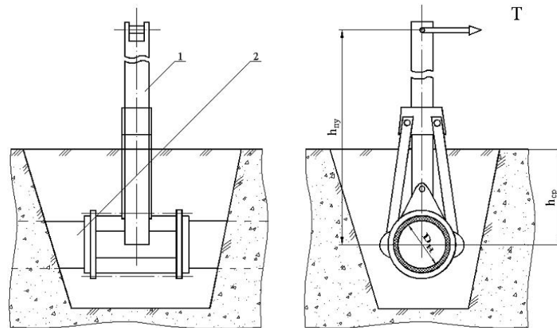
Fig. 2. The circuit of transfer of twisting moment on the underground pipeline: 1 - mounting device; 2 - the pipeline
