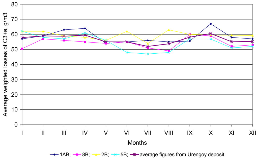
Fig.1. Total losses of C_{3+B} with separation gases
