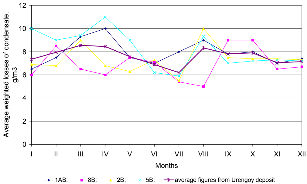
Fig.1. Total losses of C_{3+B} with separation gases
