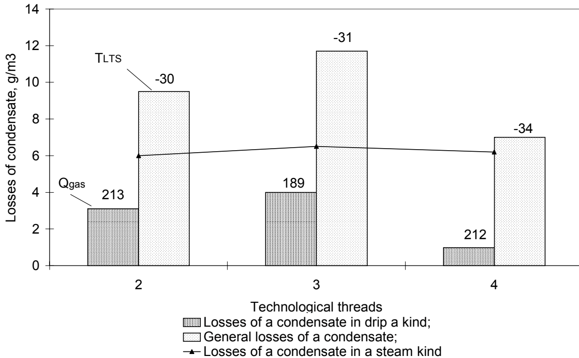
Fig.3. Losses of condensate C_{5+B} with separation gases at CIPG-5
